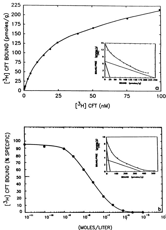
Fig. 2. Saturation of [ ^3 H]CFT binding sites measured by increasing the concentration of [ ^3 H]CFT (0.3–100 nM) (a) or by fixing the concentration of [ ^3 H]CFT (0.3 nM) and increasing the concentration of unlabeled CFT (b). Data are means of triplicate determinations of representative experiments. In a, specific binding is plotted as a function of [ ^3 H]CFT concentration. In b, the percentage of specifically bound [ ^3 H]CFT (0.3 nM) is plotted as a function of increasing concentrations of unlabeled CFT. Insets, Scatchard transformations.
